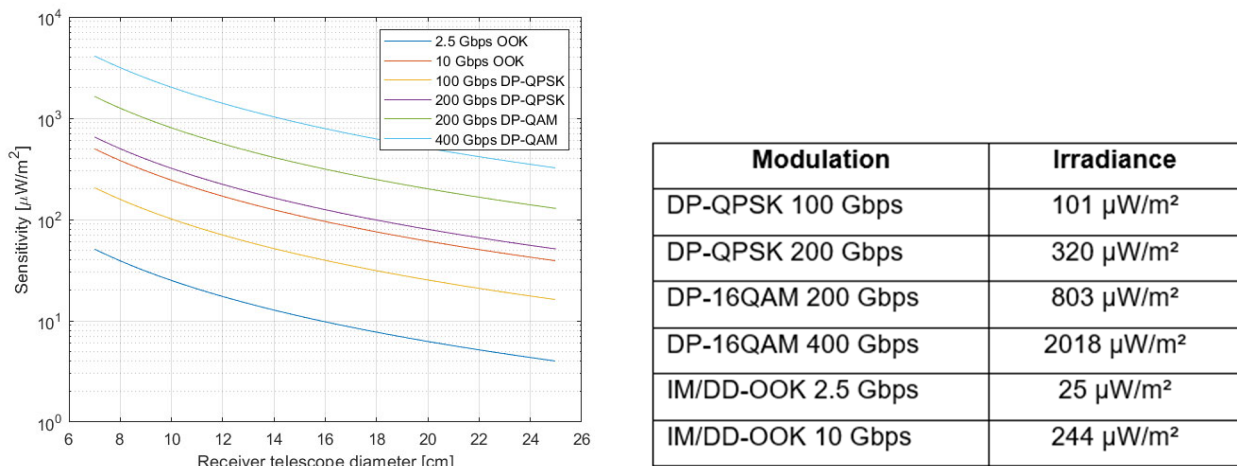
Figure 5. Left: Sensitivity at the receiver aperture depending on the receiver aperture diameter and the modulation data-rates. Right: exemplary irradiance values for a 10cm aperture diameter.
